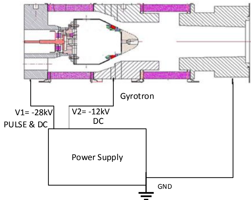
Figure 1: Schematic of test set-up using two DC supply
