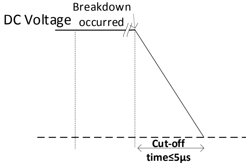
Figure 2: Typical representation of power supply's voltage behavior (DC-mode) with time during arcing/breakdown event.
