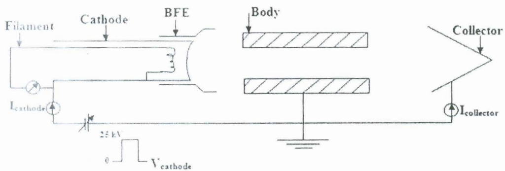
Fig1. Circuit diagram showing electrical connections on different electrodes
