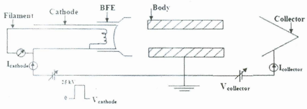
Fig2. Circuit diagram showing electrical connections on different electrodes
