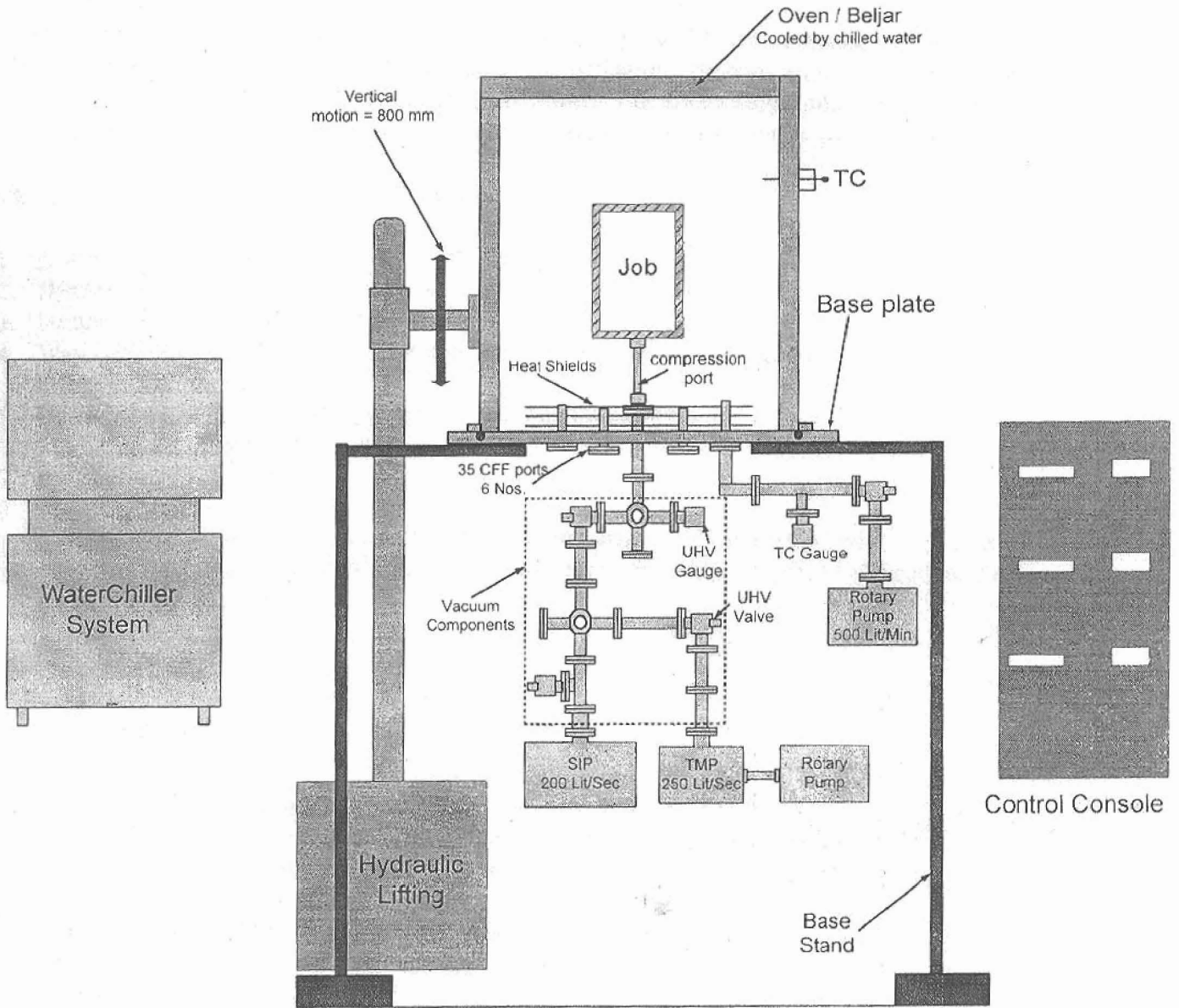
Schematic view of Vacuum Processing Unit
